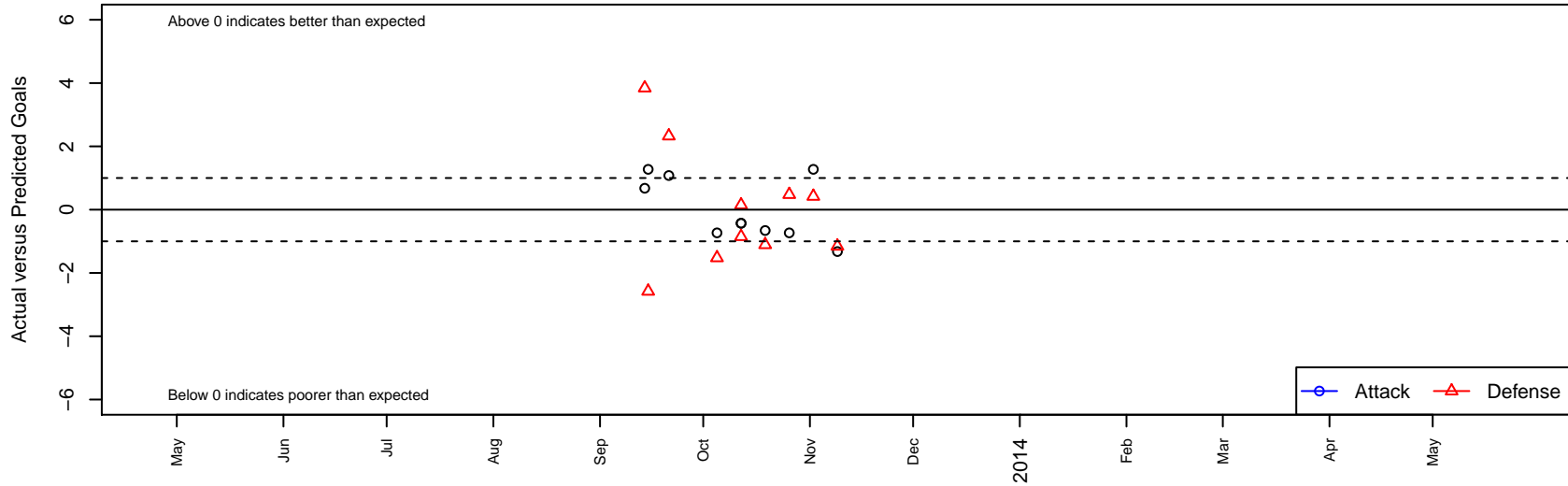
Sabers Hallock G00 Dots are actual minus expected GF (blue circles) and GA (red triangles). Blue line is smoothed change in attack strength. Red is smoothed change in defense strength.
